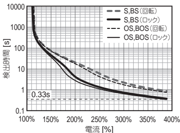
● 形 R88M-1M05030T
