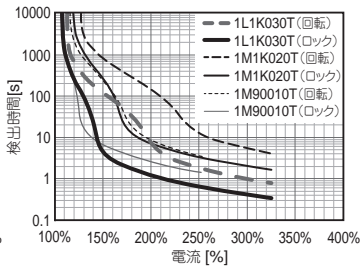
● 形 R88M-1L1K030T/-1M1K020T/ -1M90010T
