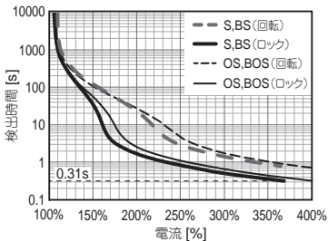
● 形 R88M-1M75030T
