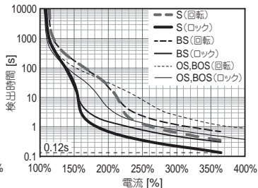
● 形 R88M-1M40030T
