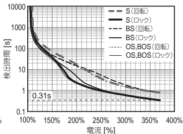
● 形 R88M-1M10030T
