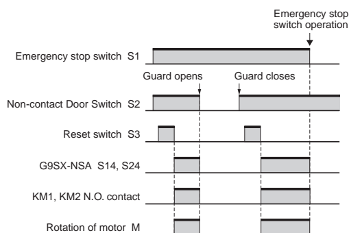
Timing chart
