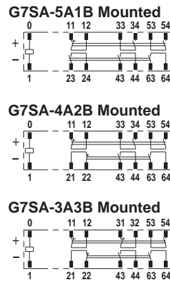
Terminal Arrangement/Internal Connection Diagram (Bottom View)
