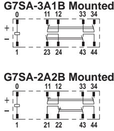
Terminal Arrangement/Internal Connection Diagram (Bottom View)
